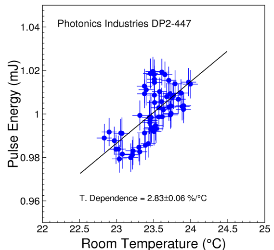
Figure 10. The temperature dependence of the laser pulse energy.
