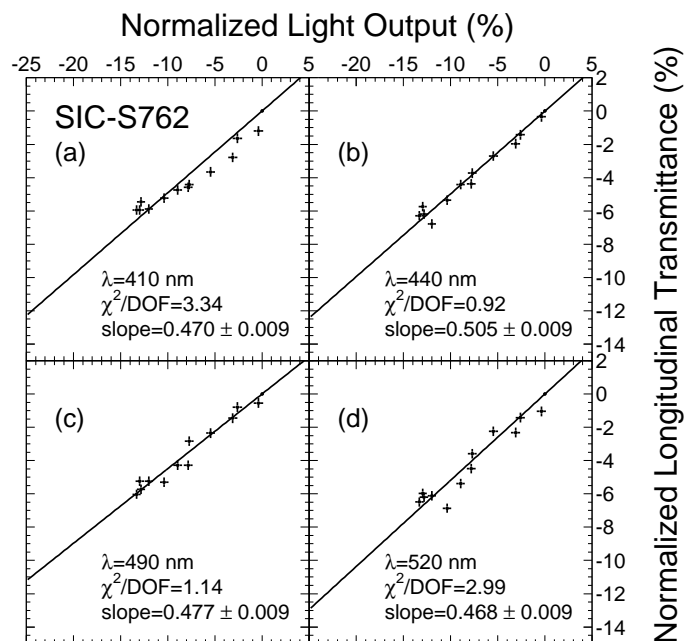
Fig. 8. Correlations between relative variations of transmittance and light output are shown at monitoring wavelength of (a) 410, (b) 440, (c) 490 and (d) 520 nm for a Y doped sample SIC-S762.
