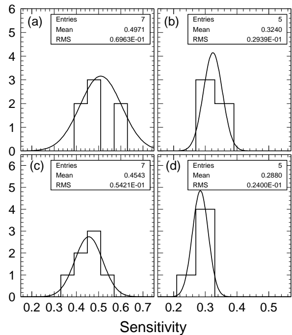
Fig. 17. Sensitivity at 440 and 490 nm is shown for the samples grown by (a) and (c) Bridgman and (b) and (d) Czochralski method, respectively.
