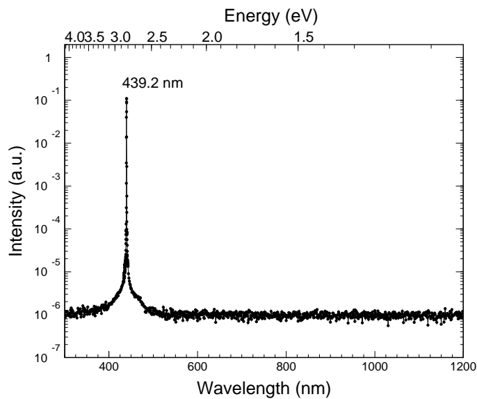
Fig. 16. Ti:Sapphire laser pulse spectrum at 440 nm is shown as a function of wavelength.
