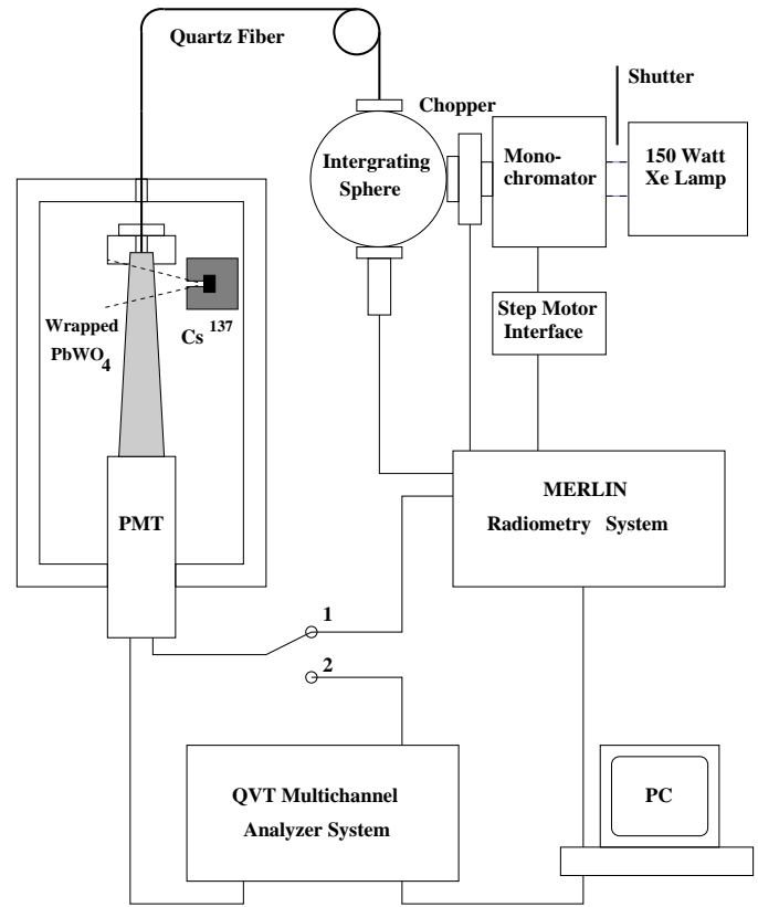
Fig. 5. The monitoring test bench for the transmittance (position 1) and light output (position 2) measurement.
