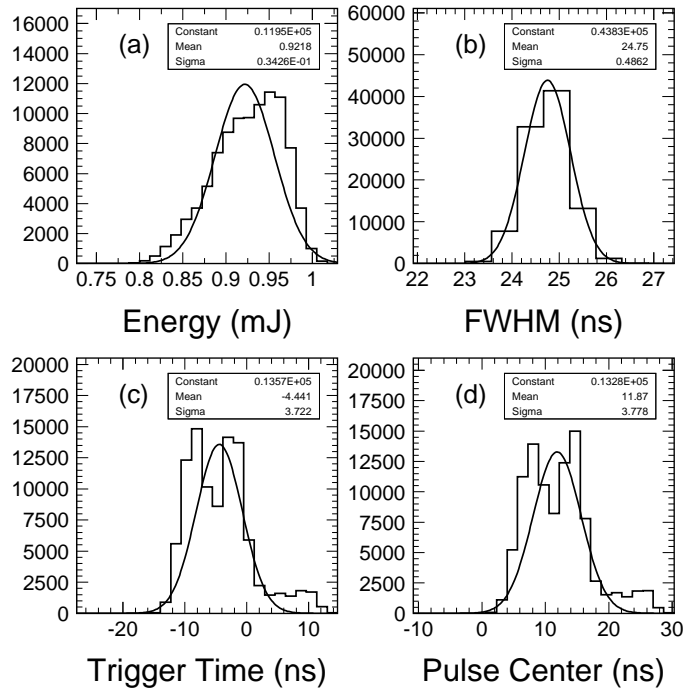
Fig. 12. Distributions of (a) pulse energy, (b) FWHM, (c) Trigger time and (d) pulse center from monitoring Ti:Sapphire laser at 440 nm, obtained in a test run of 135 hours.
