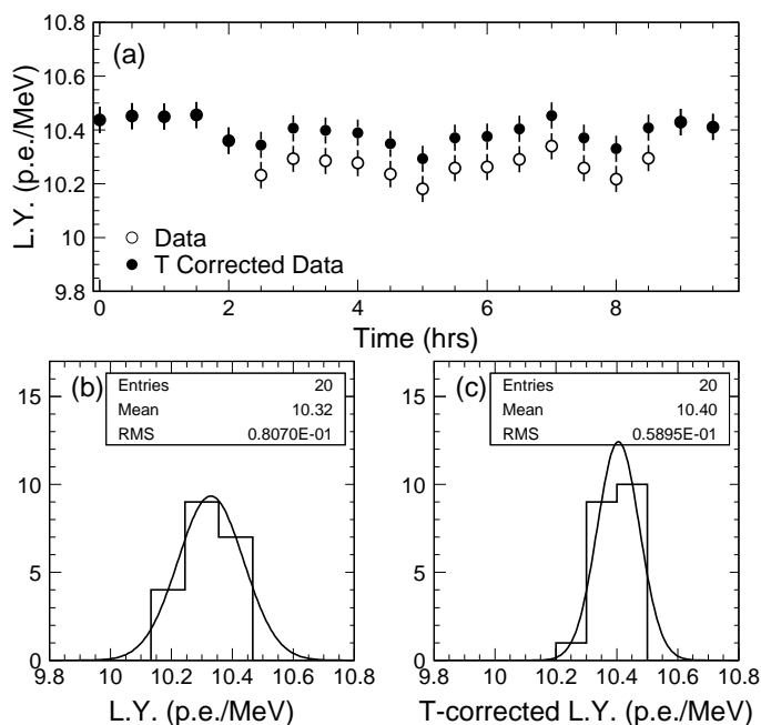
Fig. 7. (a) Light output measured by the PMT through a LeCroy QVT (position 2 in Fig. 5), taken in 9 hours, and its distributions (b) without and (c) with temperature corrections.
