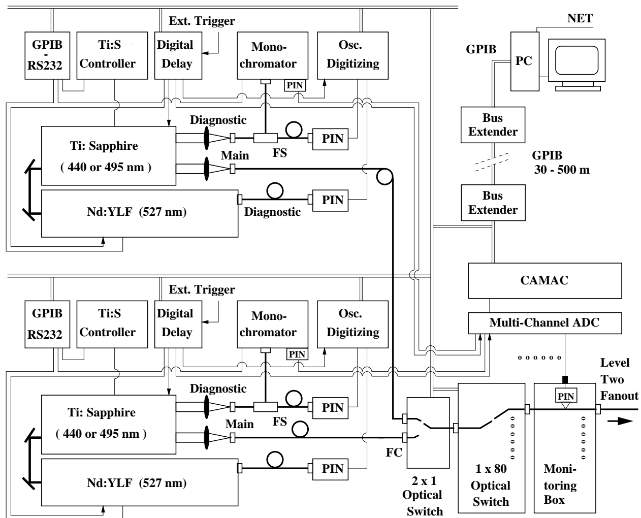
Fig. 1. The conceptual design of the monitoring light source and high level distribution system for the CMS PbWO 4 calorimeter.
