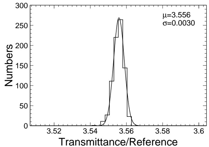
Fig. 6. Distribution of the PMT output normalized to the reference detector on the sphere (position 1 in Fig. 5), taken in 23 hours.
