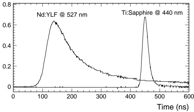
Fig. 11. The monitoring laser pulse shape for the YLF:Nd pumping laser at 527 nm and the Ti:Sapphire laser at 440 nm.
