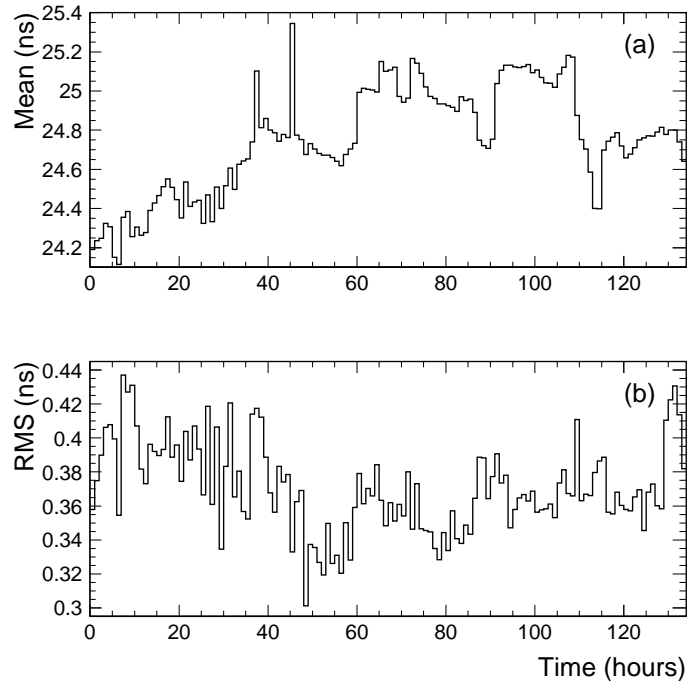
Fig. 14. The history of (a) Ti:Sapphire laser pulse width at 440 nm and (b) its standard deviation, obtained in a test run of 135 hours.
