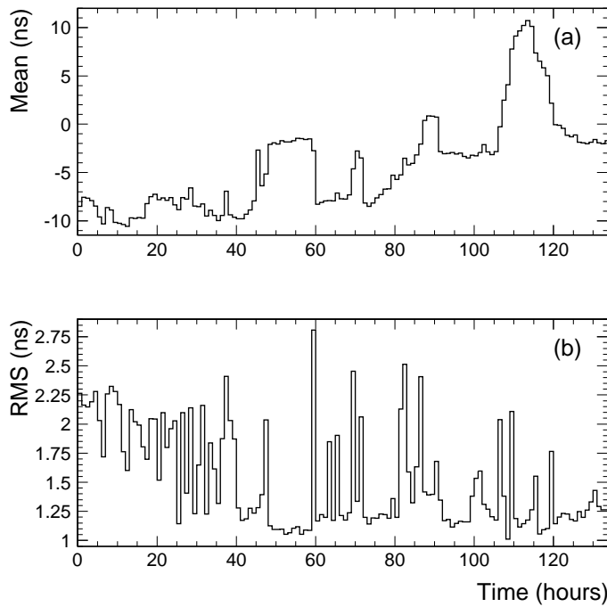
Fig. 15. The history of (a) Ti:Sapphire laser trigger timing at 440 nm and (b) its standard deviation, obtained in a test run of 135 hours.
