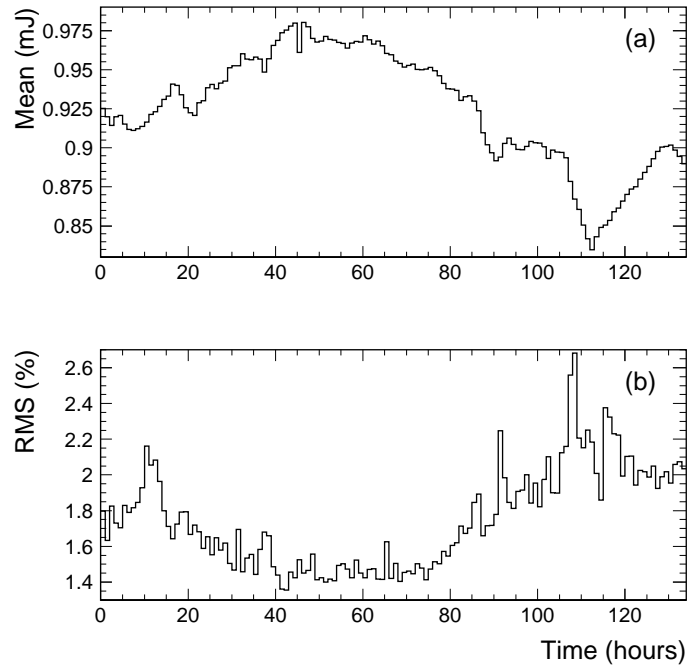
Fig. 13. The history of (a) Ti:Sapphire laser pulse energy at 440 nm and (b) its standard deviation, obtained in a test run of 135 hours.
