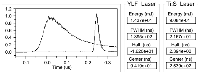
Fig. 4. The laser pulse shape display showing a wide pulse from the YLF:Nd pumping laser, a narrow pulse from the Ti:S laser and performance of two lasers.
