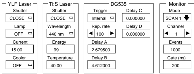
Fig. 2. The setting window showing control parameters for a Nd:YLF pumping laser, a Ti:S laser and the run control.
