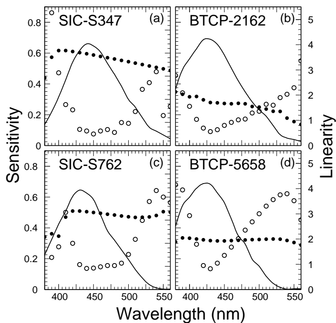
Fig. 9. Monitoring sensitivity (solid dots), linearity (open dots) and emission spectrum (solid lines) are shown as functions of wavelength for samples (a) SIC-S347, (b) BTCP-2162, (c) SIC-S762 and (d) BTCP-5658.
