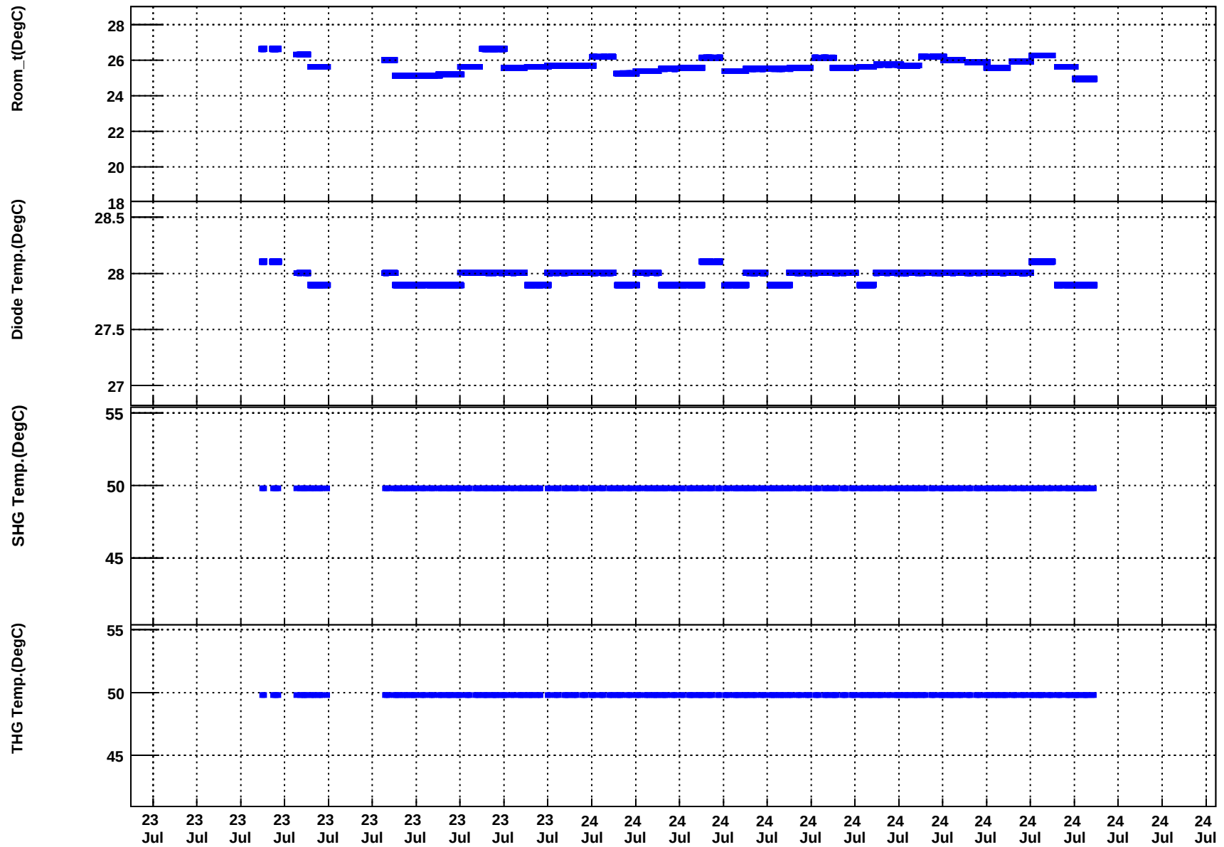
DP2-2 Temp & current
