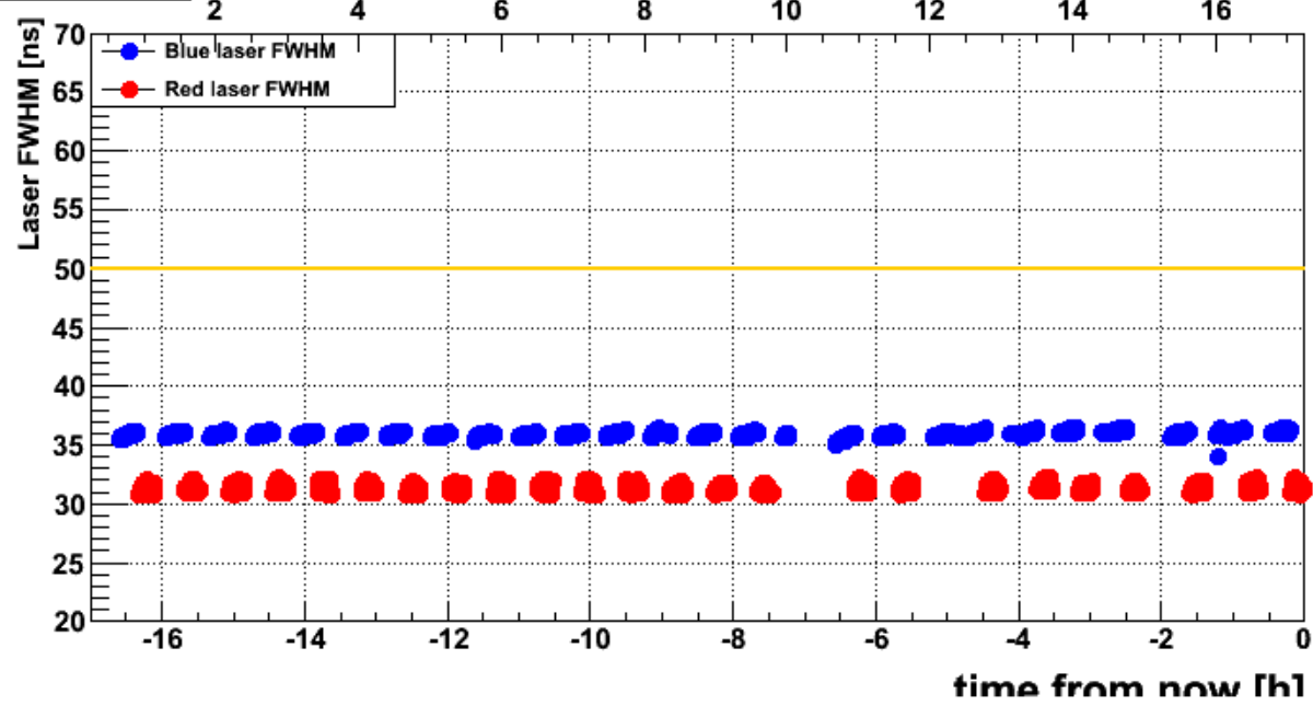
Laser FWHM
