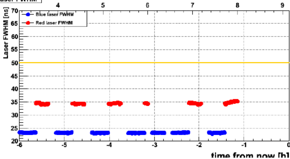
Laser FWHM
