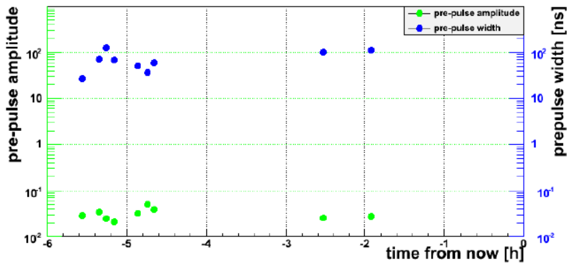
Pre-pulse search
