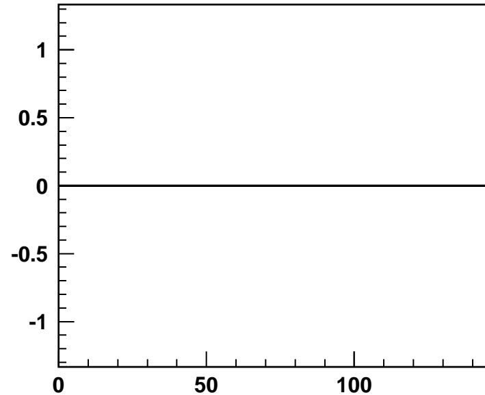
Chan 66
