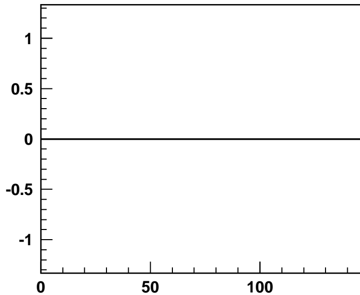
Chan 71
