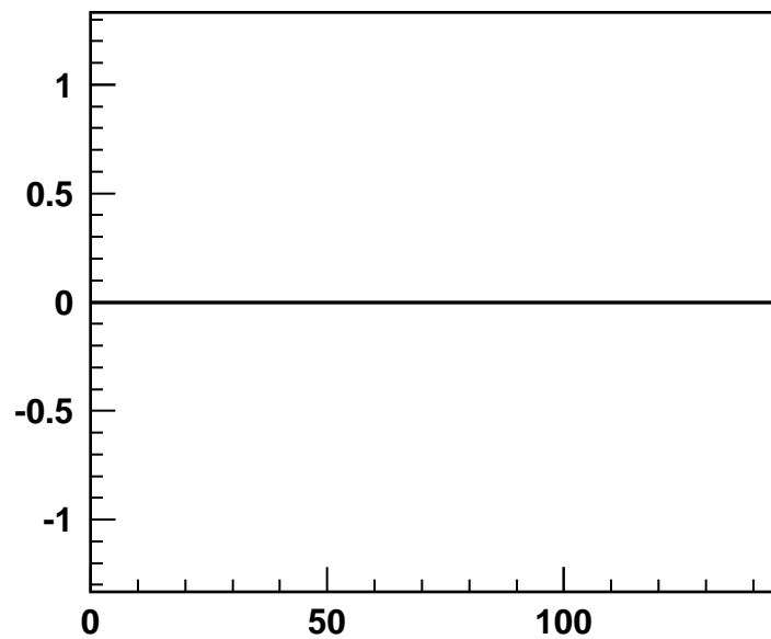
Chan 60
