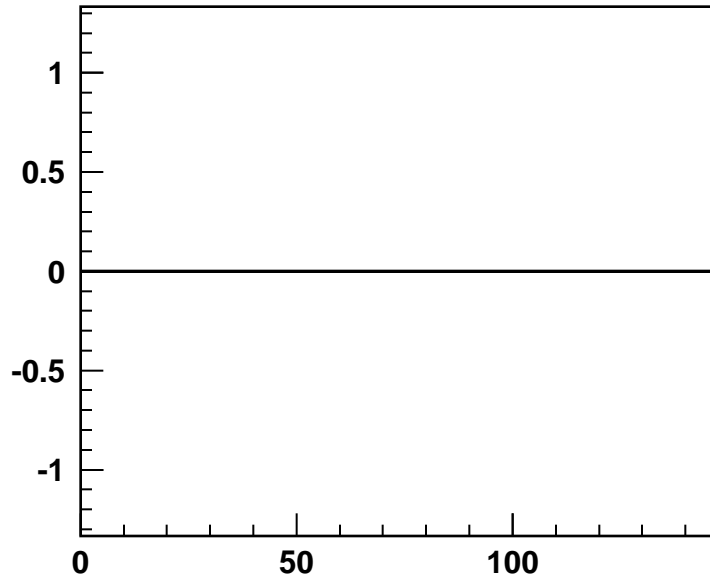
Chan 57
