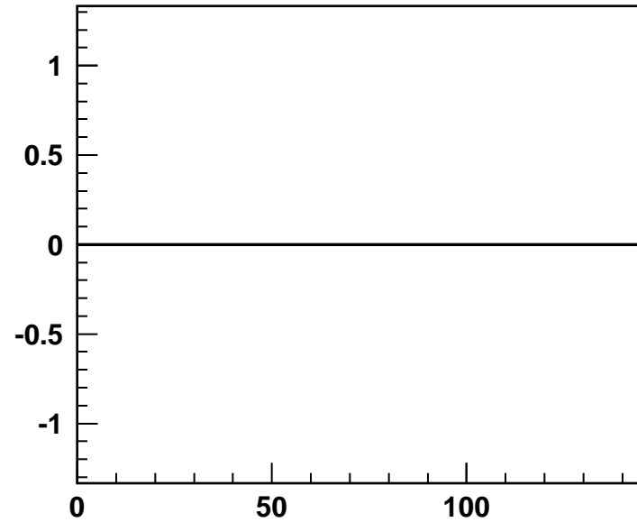
Chan 82
