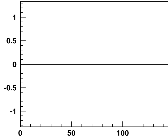
Chan 42
