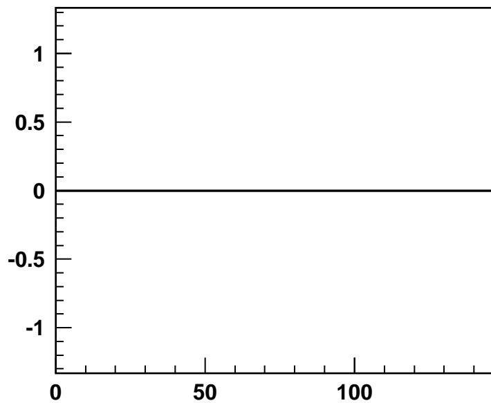
Chan 67
