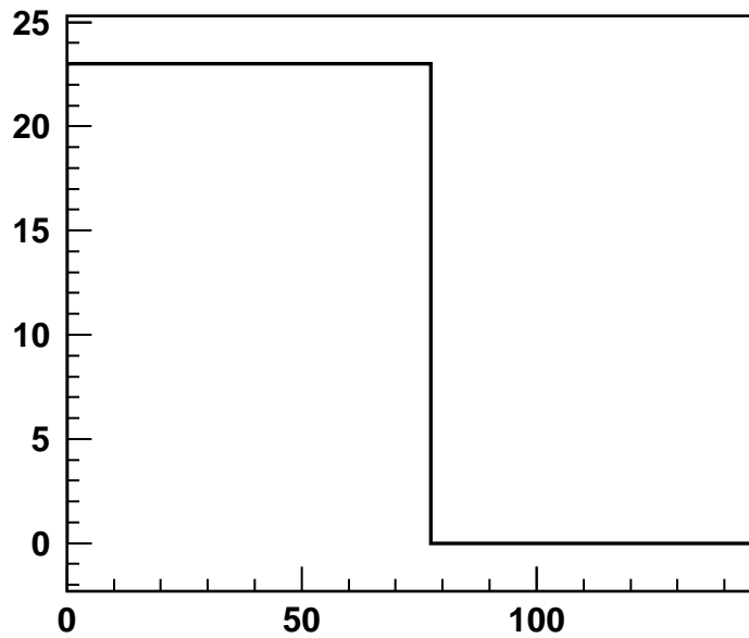
Chan 81
