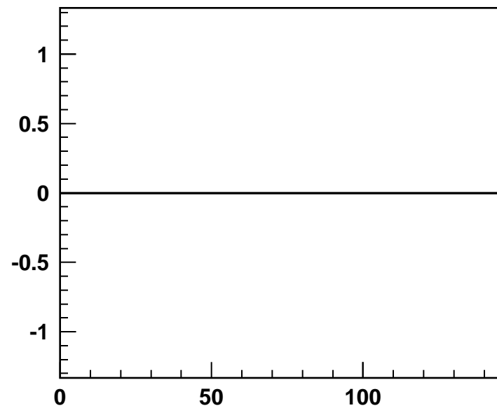
Chan 68
