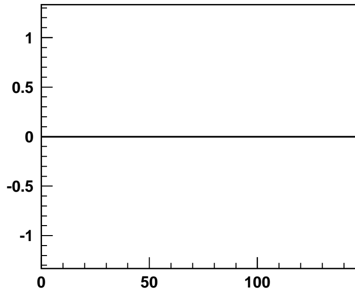
Chan 64
