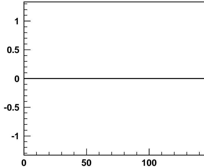
Chan 58
