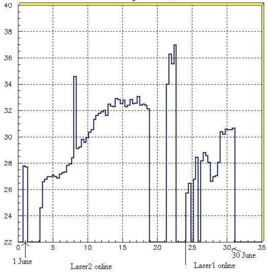
FWHM History 440nm June2004
