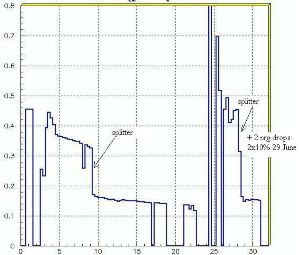
TIS: Energy History 440nm
