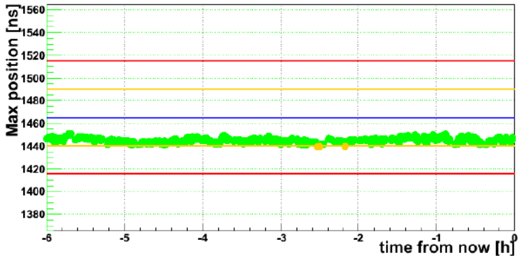
Laser timing
