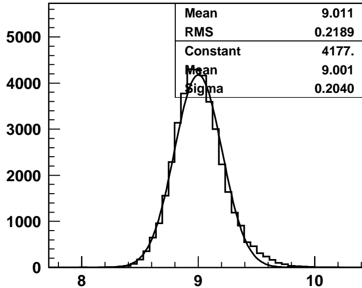
Energy
