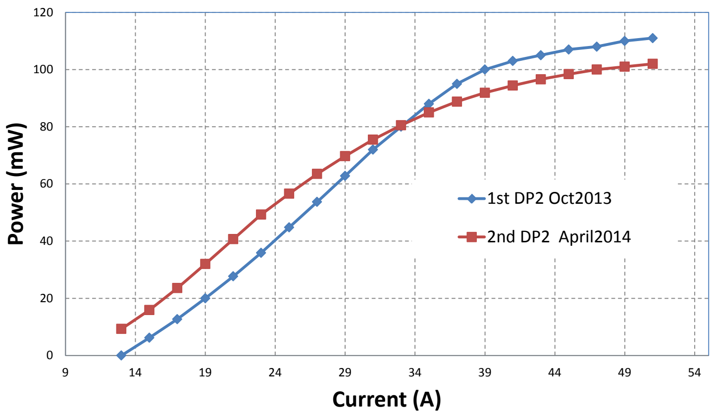
The 1st (SN:11-381) and 2nd (SN:12-658) DP2-7 Lasers
