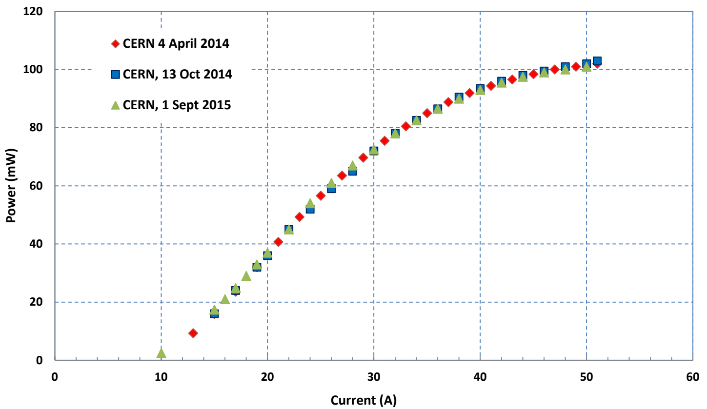
The 2nd DP2 laser (SN:12-658) output power
